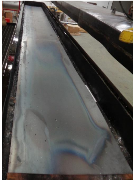
Photo No. 3 Unexposed Surface of the Test Specimen (Post-test)
