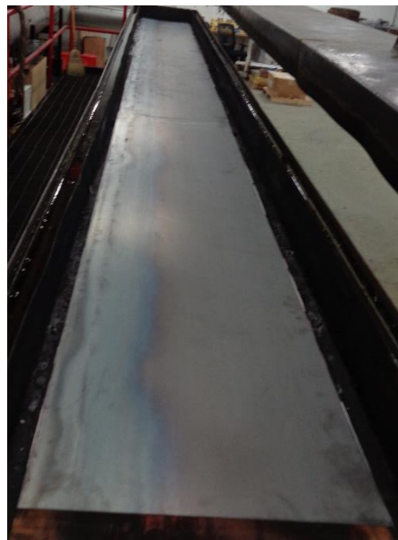
Photo No. 2 Unexposed Surface of the Test Specimen (Pre-test)
